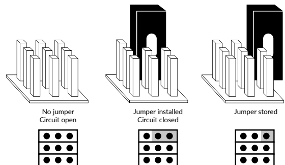
Figure 3 - Jumper installation
