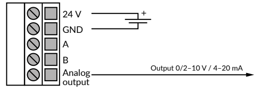
Figure 2b - Wiring diagram: Power input & signal output
