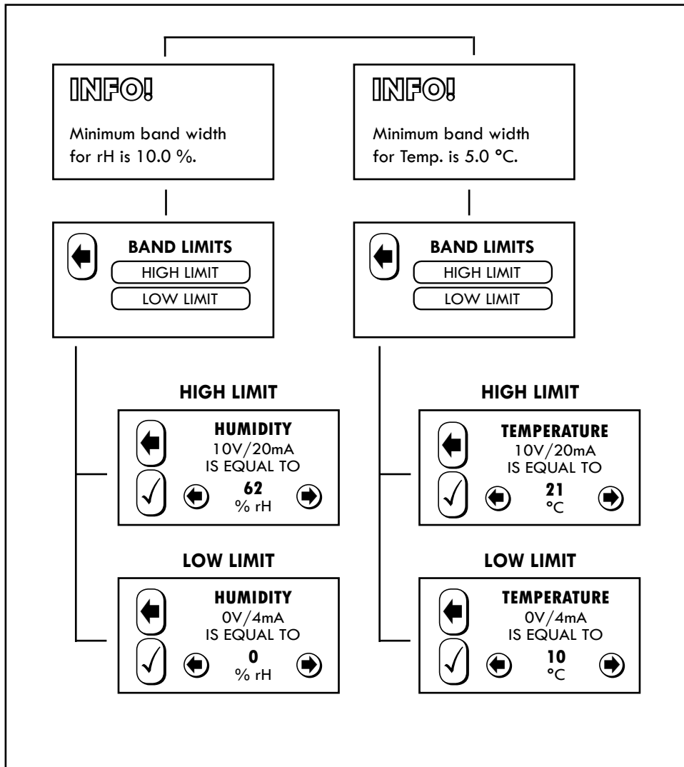
Figure 9 - P-Bands
